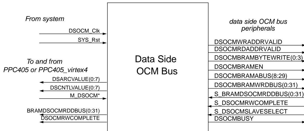
Figure 1: Data Side OCM Bus Block Diagram
