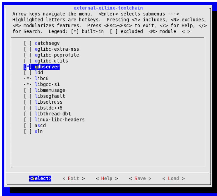
Figure 8: external-xilinx-toolchain sub-menu
