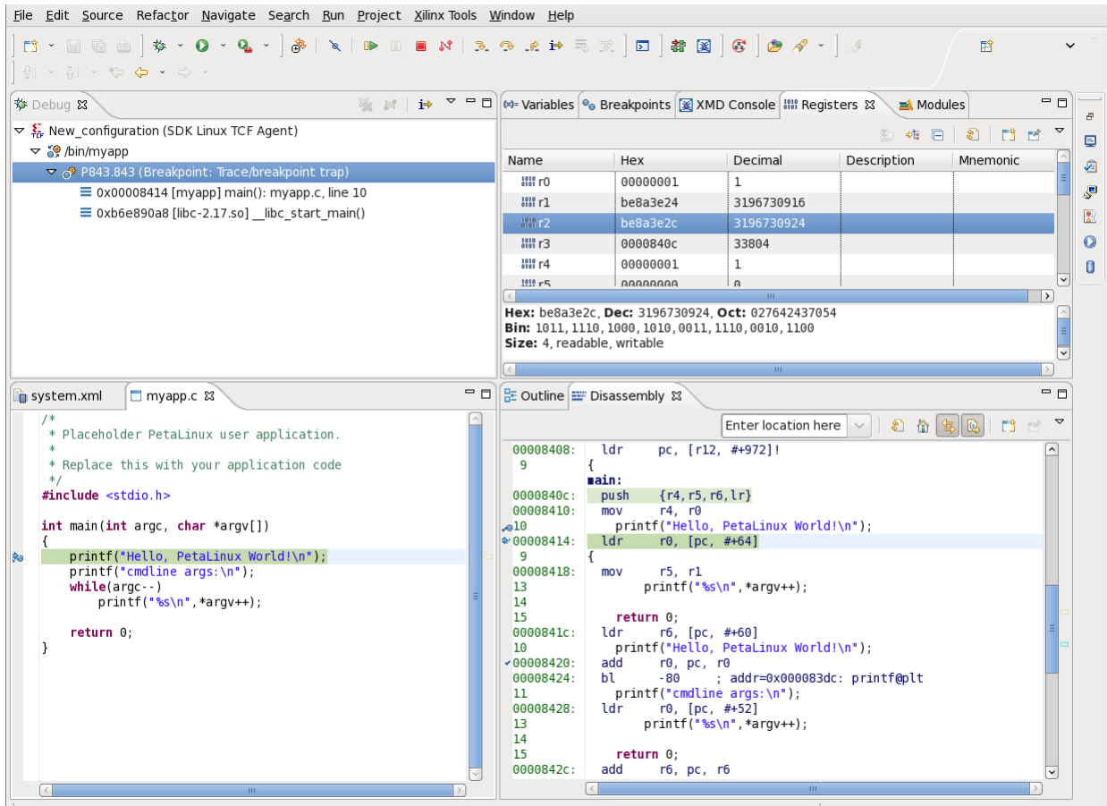
Figure 4: XSDK Debug
