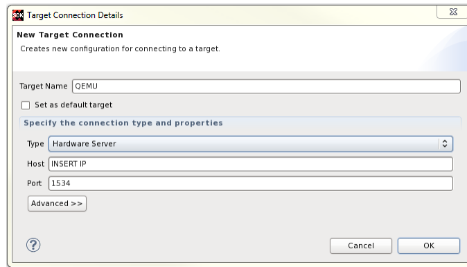
Figure 2: XSDK Debug New Target Configuration
