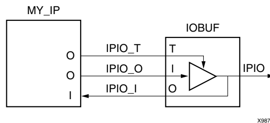
Figure 3-1: IOBUF Implementation
