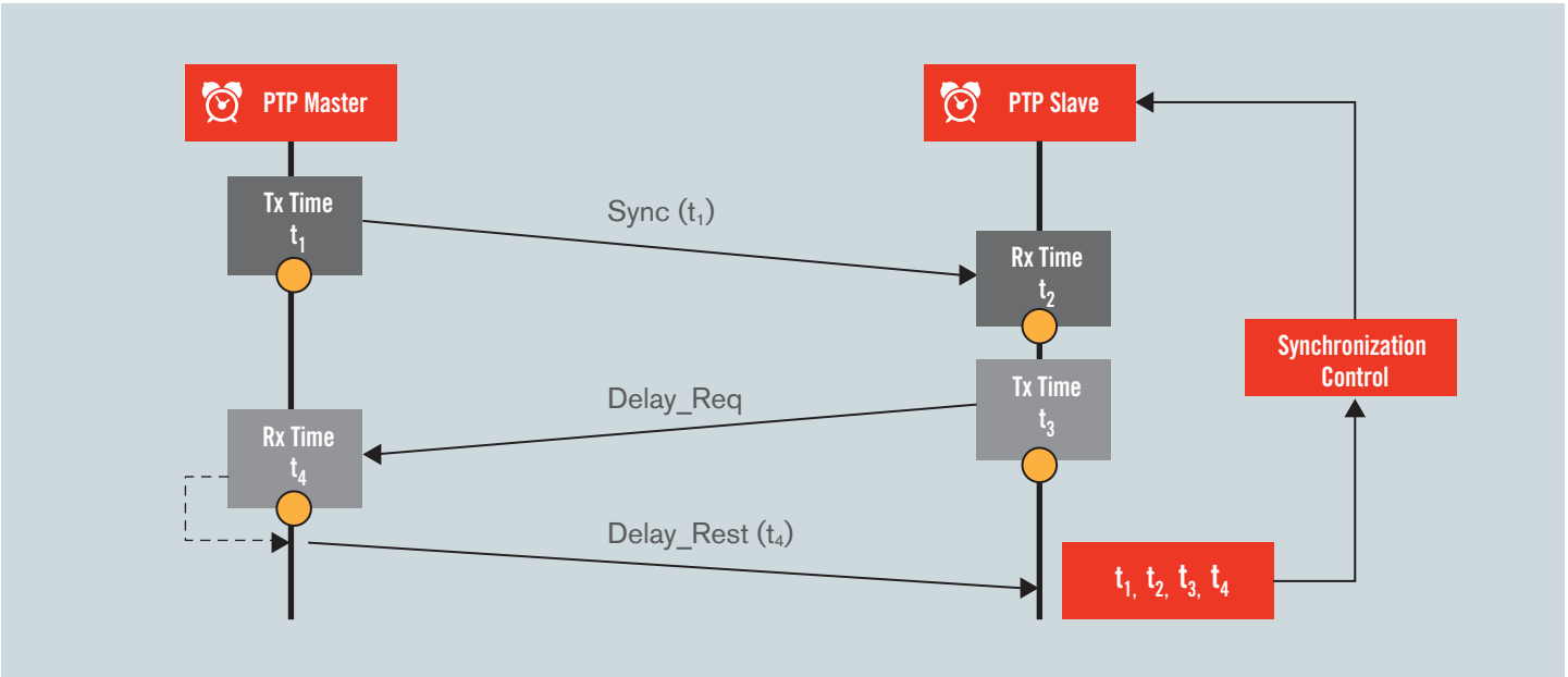
Figure 3 IEEE1588 synchronization messages and timing
