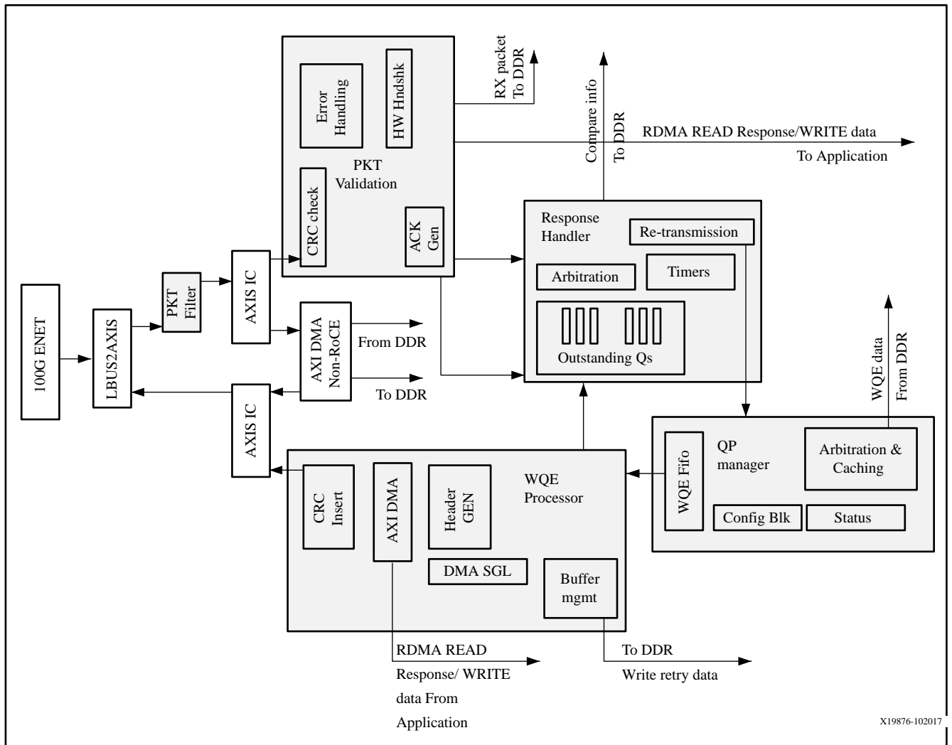
Figure 1: ERNIC IP and Subsystem
