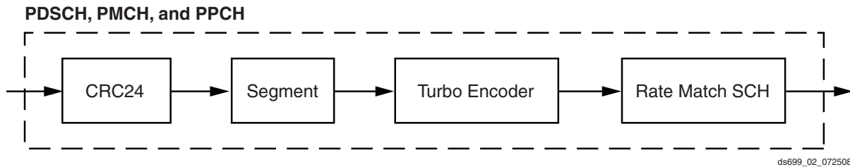
Figure 2: Downlink Channel Processing for DL-SCH, PCH and MCH -SCH Channel Stream
