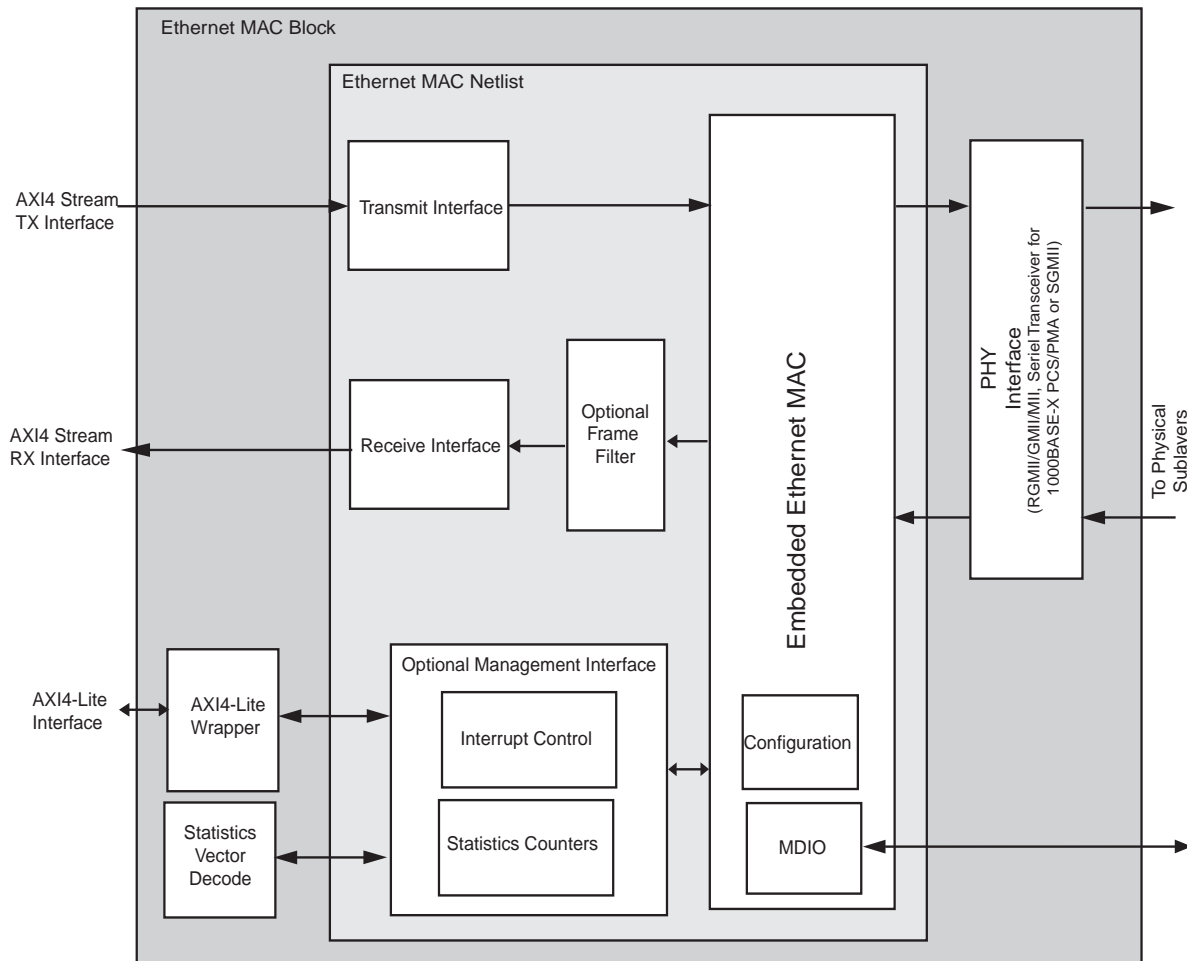
Figure 4: Virtex-6 Embedded TEMAC Functional Block Diagram
