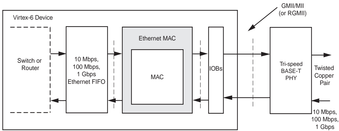
Figure 2: Typical BASE-T Application for Virtex-6 FPGA Embedded TEMAC Core
