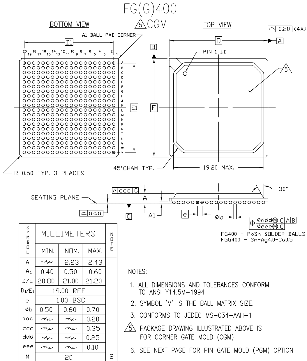
Figure 1: Corner Gate Mold Option, FG400/FGG400 Package
