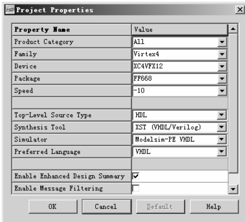
Figure 22: New Project - Device and Design Flow
