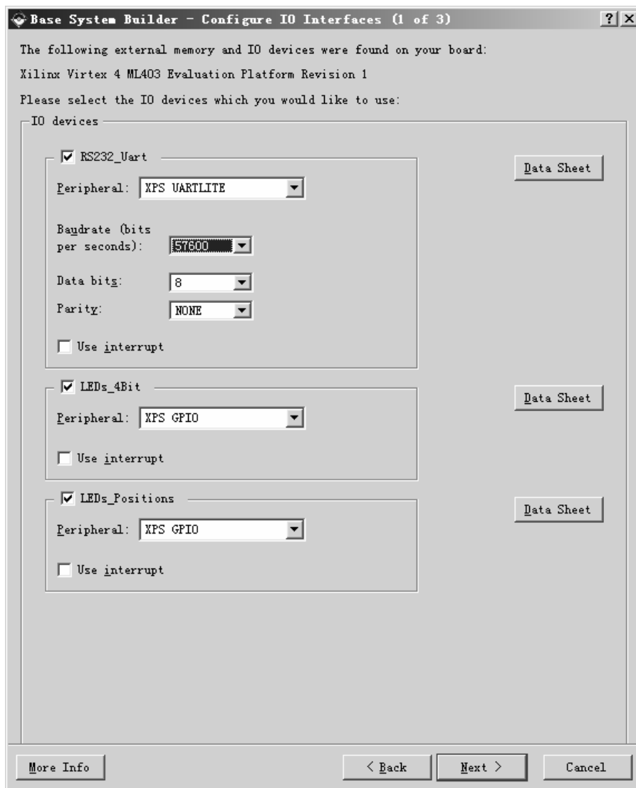
Figure 4: Configure I/O Interfaces
