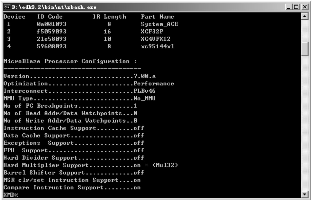
Figure 31: XMD Window
