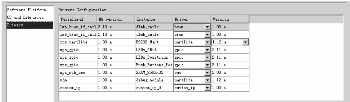
Figure 26: Drivers view
