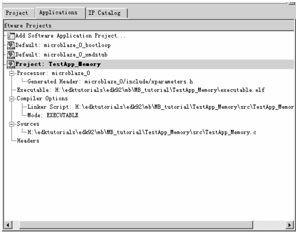
Figure 28: Applications Tab
