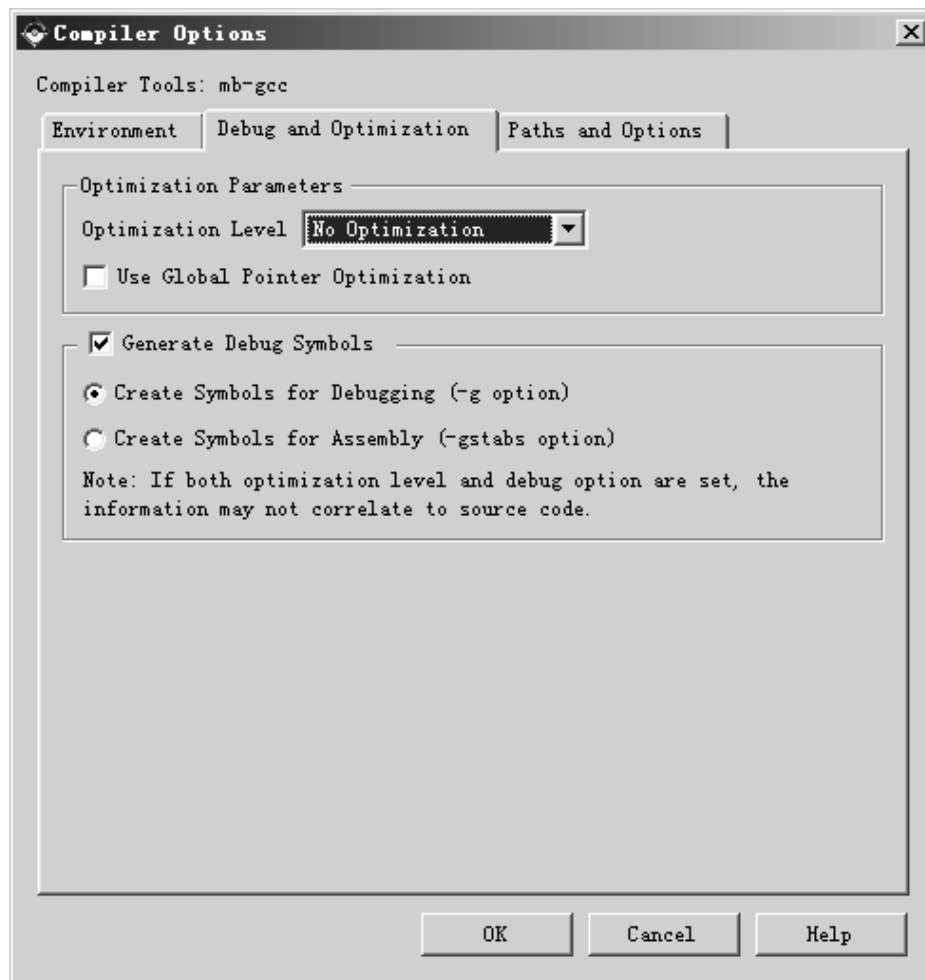
Figure 33: Compiler Options
